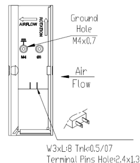
Terminal Type (T)
