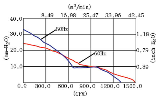
SK280 P-Q Curves
